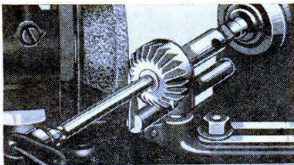
Above: Grinding a cutter with spring stop in holding fixture. Right: Grinding spiral reamer.
